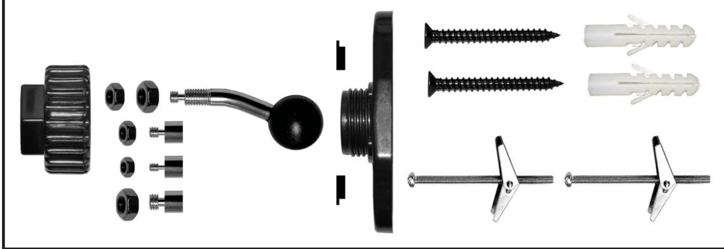
ELSPM-01: Complete kit for mounting 1 speaker
