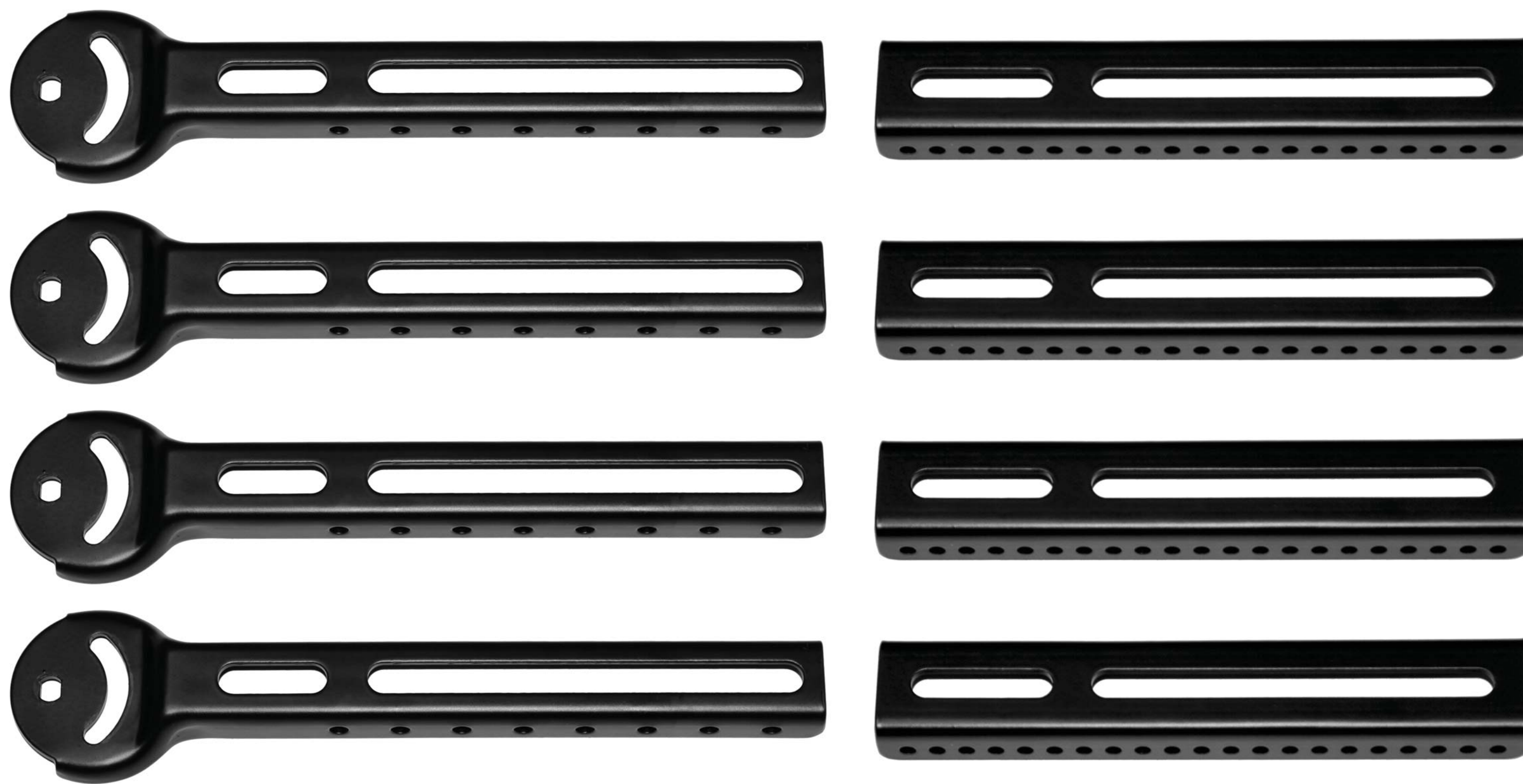
ELBA-2: 4 each of two Piece Bayonet Arm for Medium Single Stud Mount with hardware to connect the two arms plus hardware to attach to butterfly
